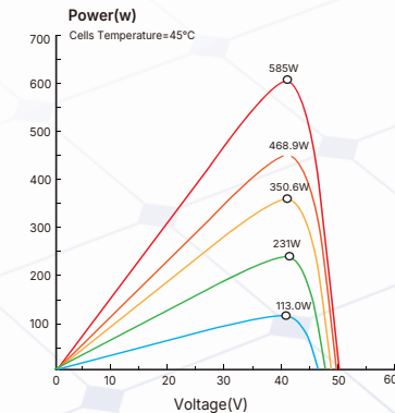
Power-Voltage Curve(620W)
