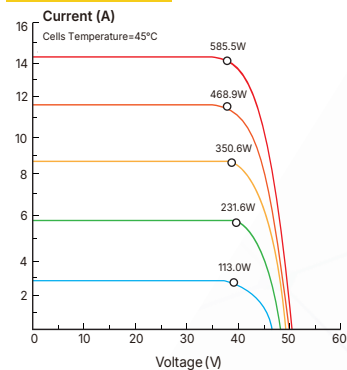
Current-Voltage Curve(610W)
